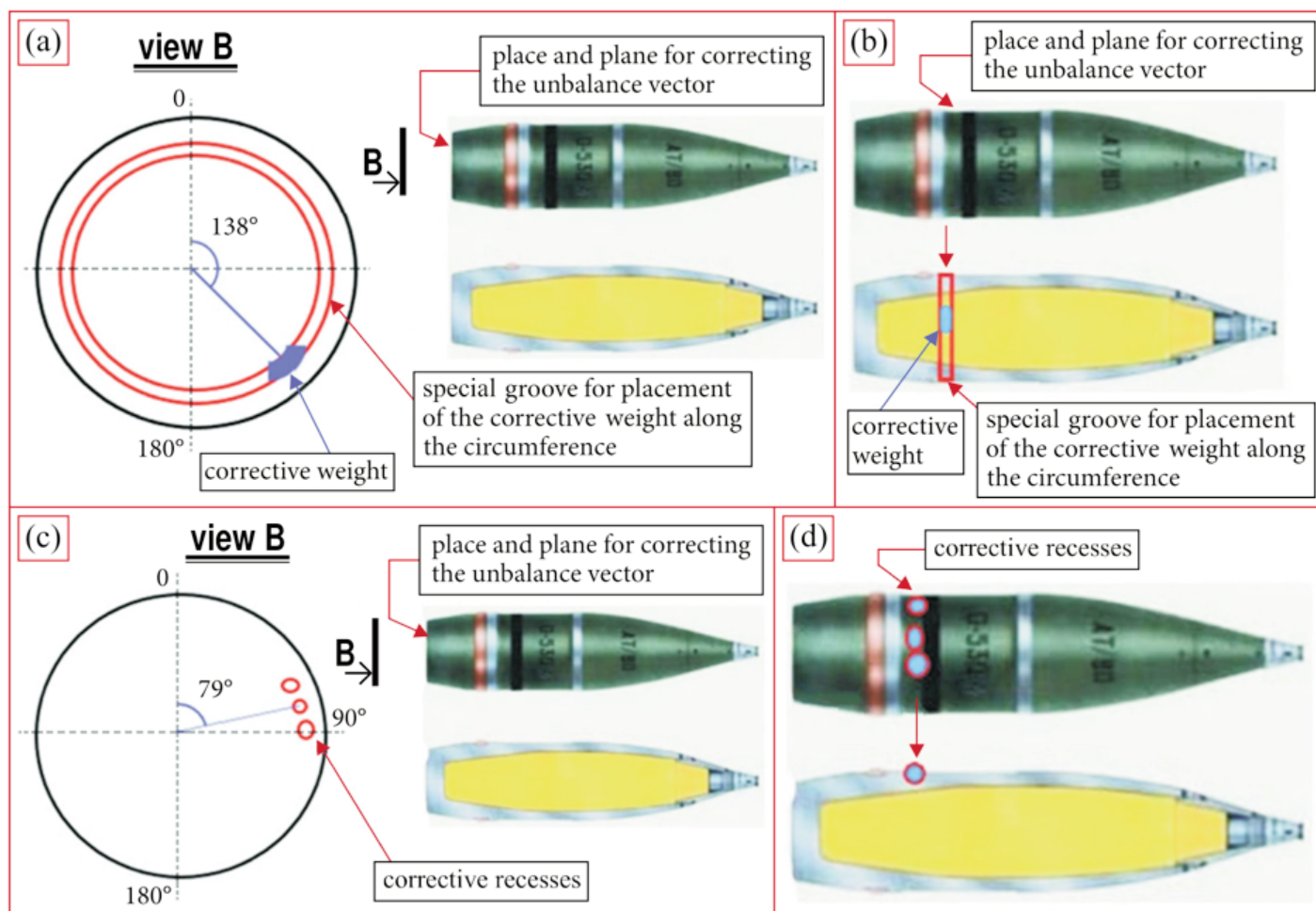
Figure 2. Versions of correcting the unbalance of the projectile: (a) and (b) by adding metal mass through a corrective weight placed in the groove in the end rear part and on the lateral surface, respectively; (c) and (d) by removing the mass of excess metal through milling in the end rear part and on the lateral surface, respectively
